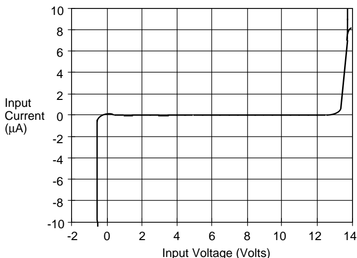
Figure 3, Input Impedance
