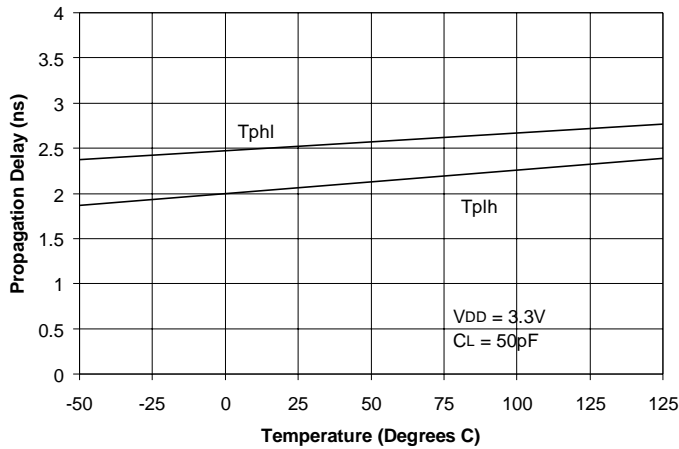
Figure 40, Delay vs. Temperature in an ALVC162244
