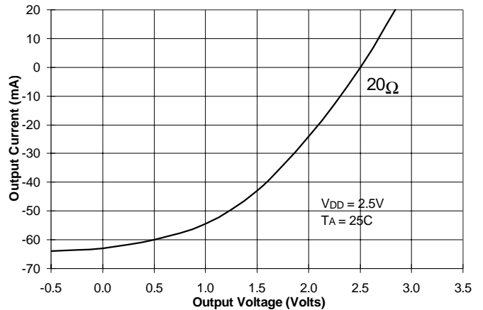
Figure 15, V OH Characteristics of ALVC16xxx at V DD = 2.5V
