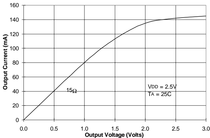
Figure 14, V OL Characteristics of ALVC16xxx at V DD = 2.5V
