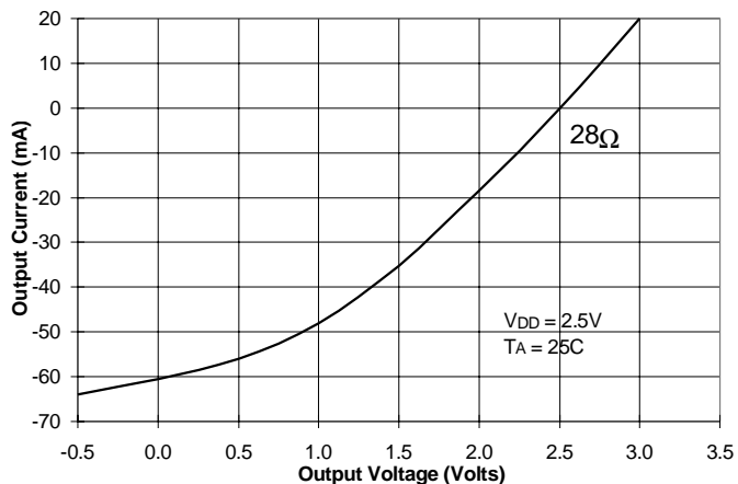
Figure 20, VoH Characteristics of ALVC162xxx at VDD = 2.5V
