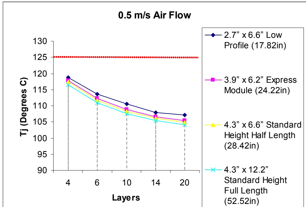
Figure 4 PES24T3G2 Heat Sink Requirements with Air Flow
