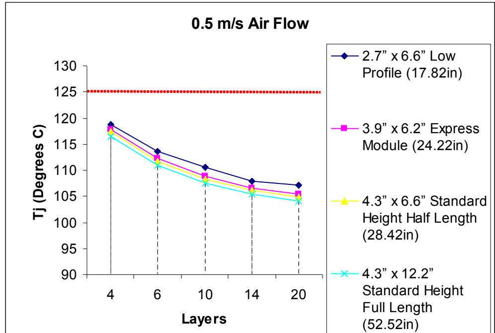
Figure 10 HI0524G2PS Heat Sink Requirements with Air Flow
