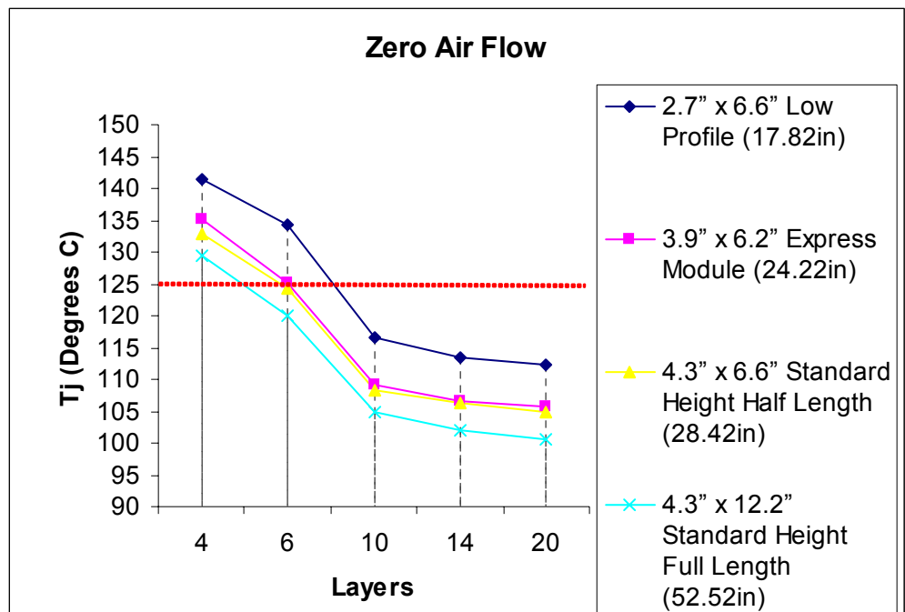
Figure 5 PES24T3G2 Heat Sink Requirements without Air Flow
