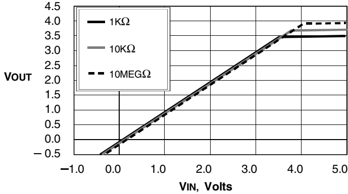
Figure 3. Typical V_{OUT} vs. V_{IN} for Various Loads
