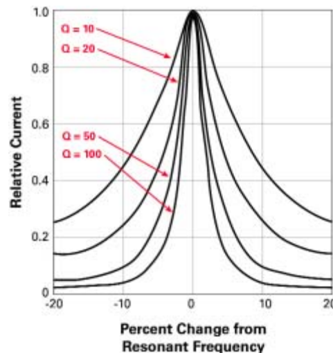
Figure 3: Q-factor percentage
