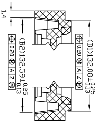
SECTION J-J
