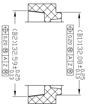
SECTION J-J
