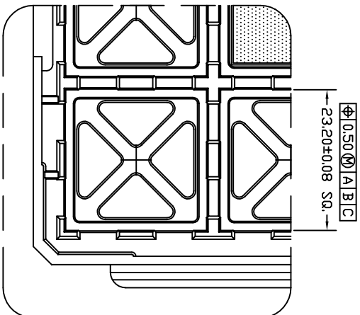
BOTTOM VIEW DETAIL "B" SCALE : 3/1 (FROM SHT.#1)
