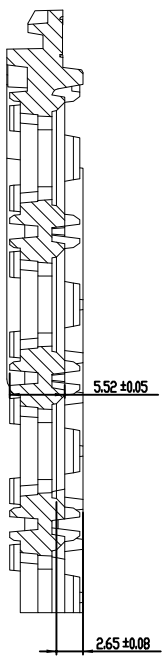
SECTION G-G
