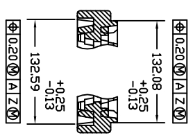
SECTION "X-X" SECTION "Y-Y" TRAY STACKING DETAIL SCALE : 3/1
