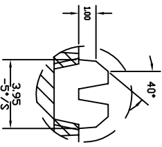
DETAIL "L" SCALE : 10/1
