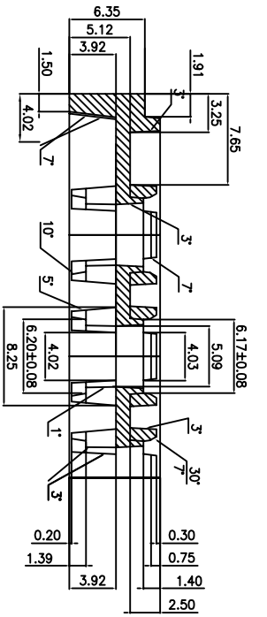
SECTION "B-B" (SCALE:4/1)
