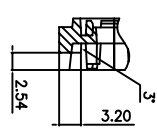
SECTION "N-N" (SCALE:2/1)
