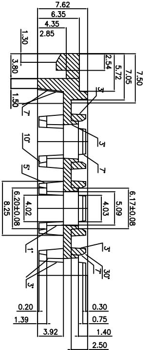
SECTION "A-A" (SCALE:4/1)
