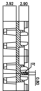
SECTION "B-B" (SCALE:4/1)
