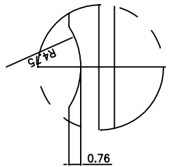
DETAIL "K" (SCALE:5/1)
