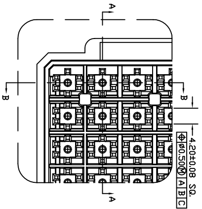
TOP VIEW DETAIL "B" SCALE : 3/1 (FROM SHIT.#1)
