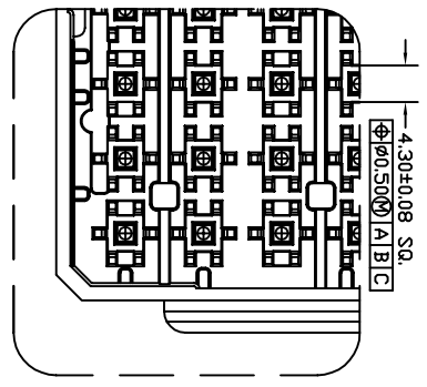
BOTTOM VIEW DETAIL "B" SCALE : 3/1 (FROM SHIT.#1)
