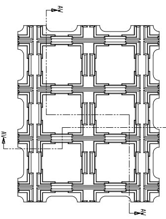
WINDOW CELL DETAIL
