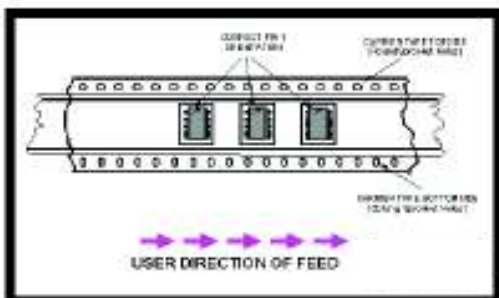
For Rectangular 2-Side Led / SOI Packages
