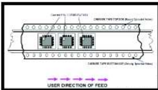
For Square 4-Side Leaded Packages
