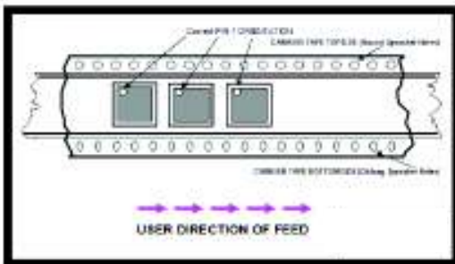
For Square BGA/QFN/COL/CLCC/LGA/WLCSP Packages
