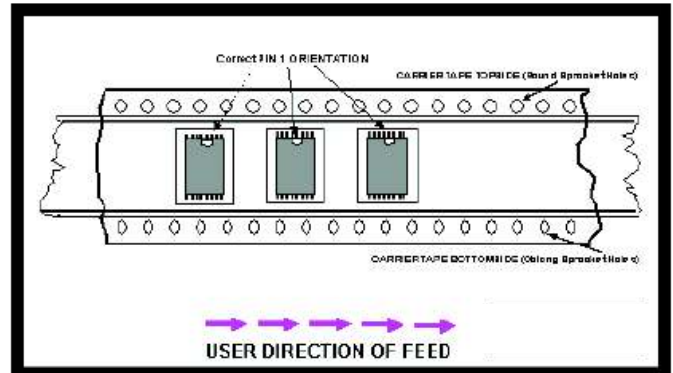
For TSOP Type I Packages
