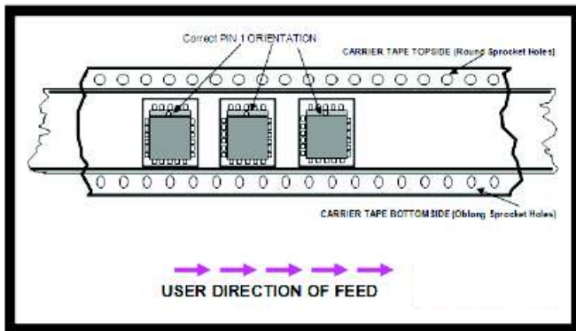
For PLCC Packages
