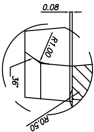
DETAIL "G" (SCALE:10/1)
