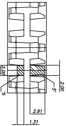
ANTI-CRUSH (SCALE:5/1)
