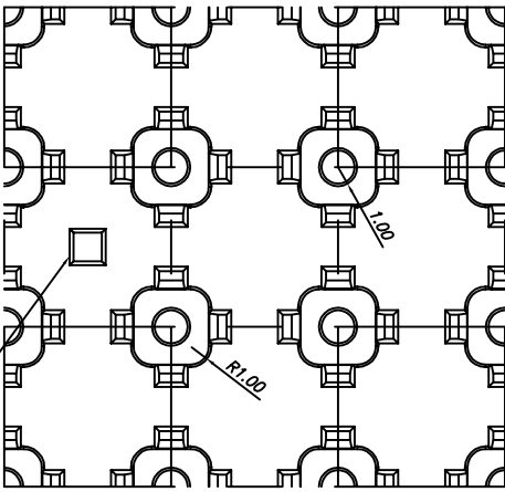
TOP VIEW (SCALE:5/1)
