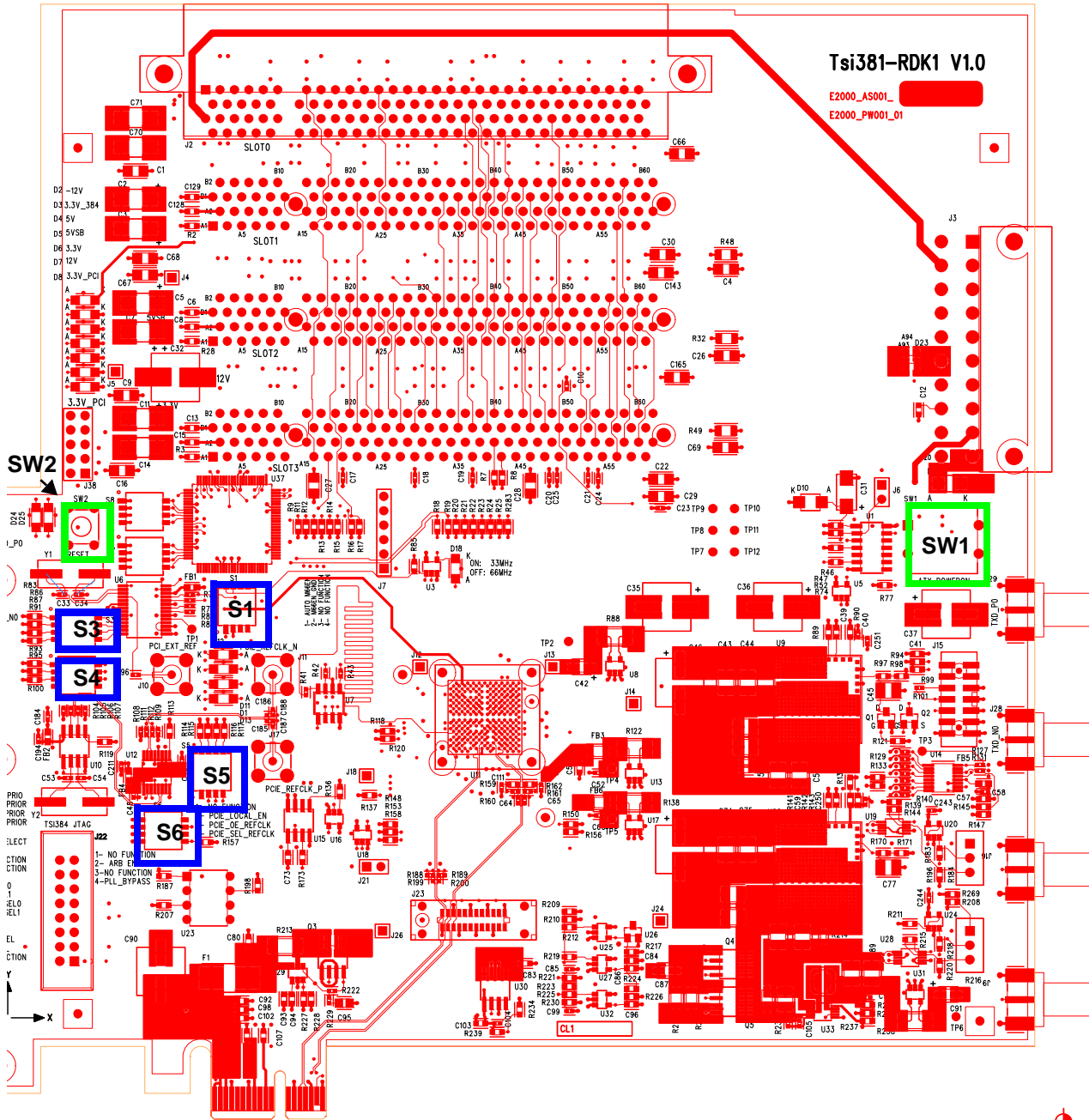
Figure 6: Switch Locations
