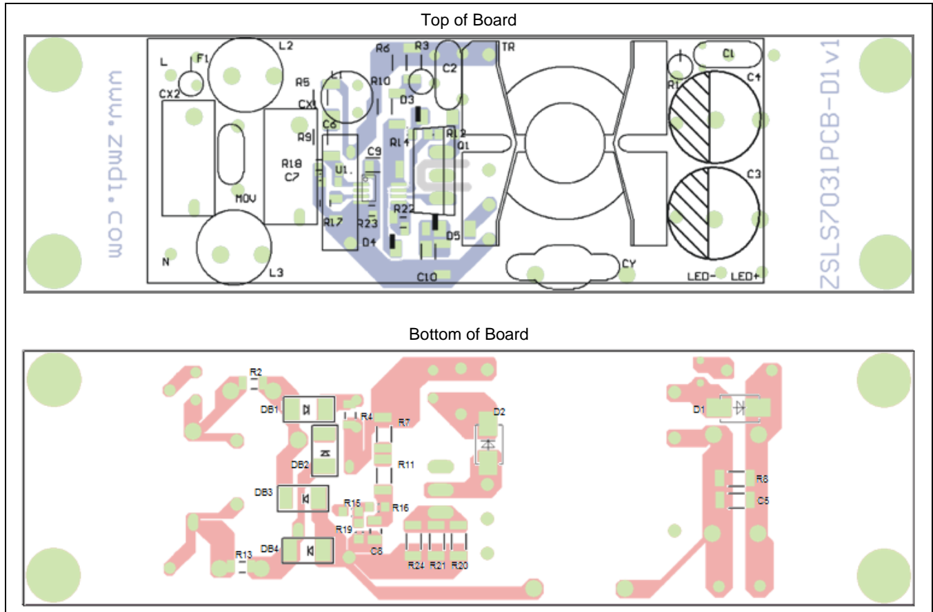
Figure 3.2 ZSLS7031PCB-D1 Demonstration Board Layout
