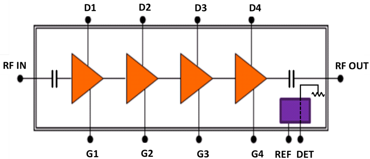
Figure 1: Device diagram
