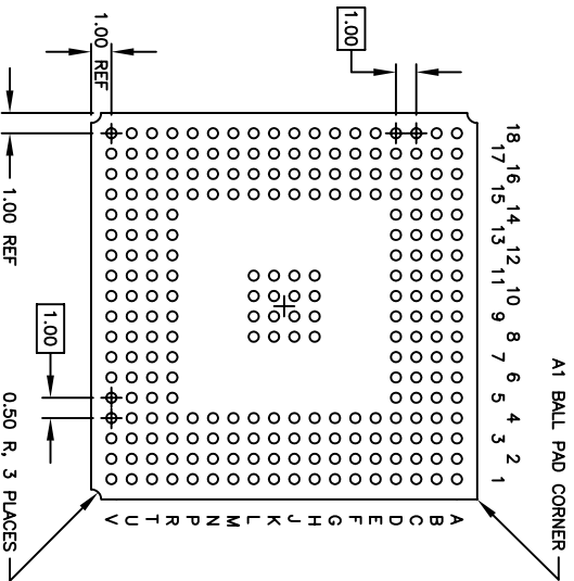
BOTTOM VIEW 240 SOLDER BALLS
