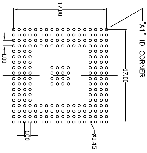
240 SOLDER BALLS
