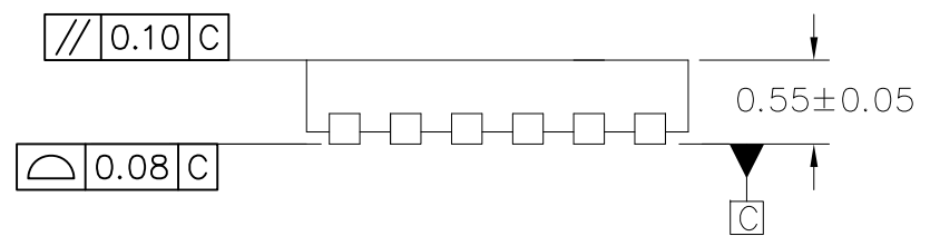
SIDE VIEW (ROTATE 90 Deg.)
