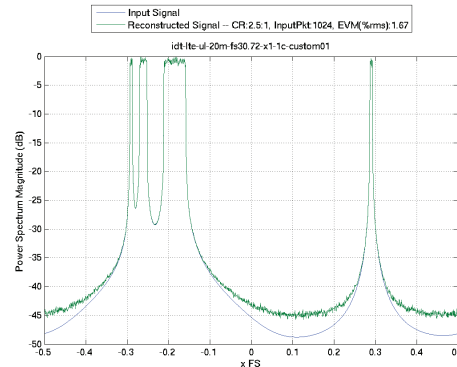
OUTPUT SIGNAL SPECTRUM
