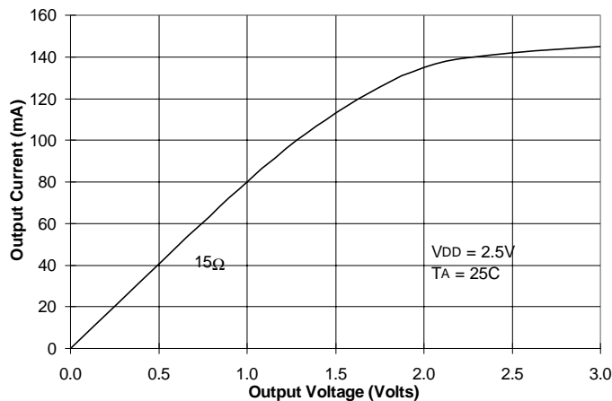
Figure 14, VOL Characteristics of ALVC16xxx at VDD = 2.5V
