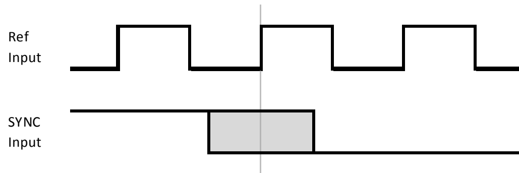
Figure 4. SYNC Input Sampling – On Target (Default)
