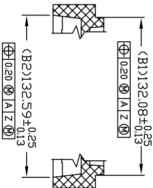
SECTION J-J
