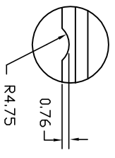
DETAIL C
