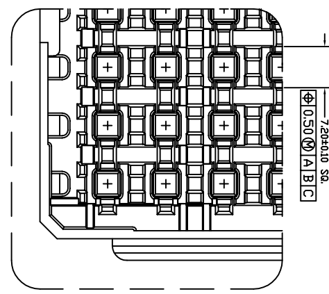
BOTTOM VIEW DETAIL "B" SCALE : 3/1 (FROM SHT.#1)
