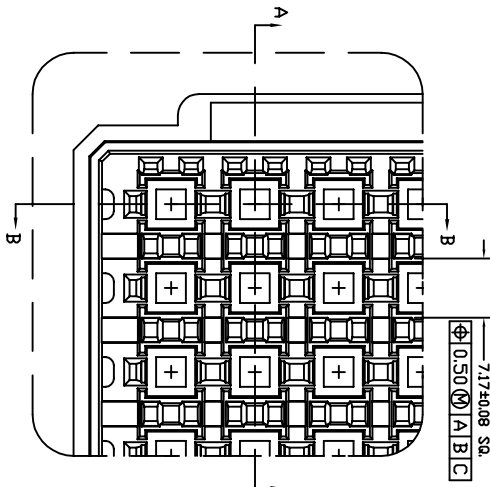
TOP VIEW DETAIL "B" SCALE : 3/1 (FROM SHT.#1)
