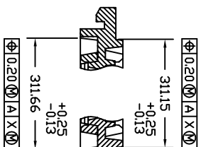
SECTION "X-X" TRAY STACKING DETAIL SCALE : 3/1
