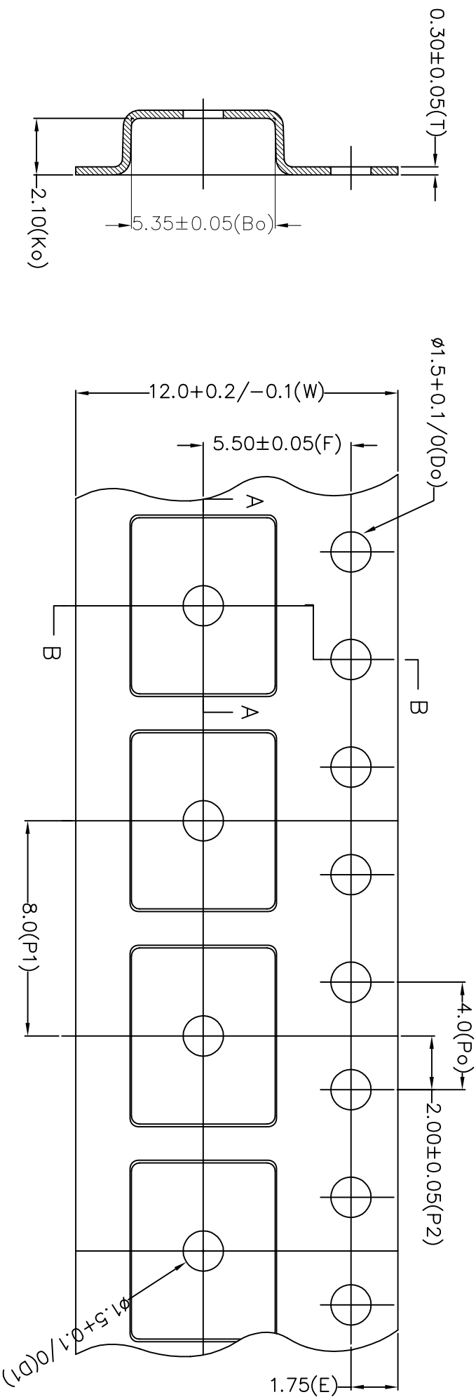
Section B-B
