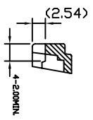
SECTION D - D(1:1)
