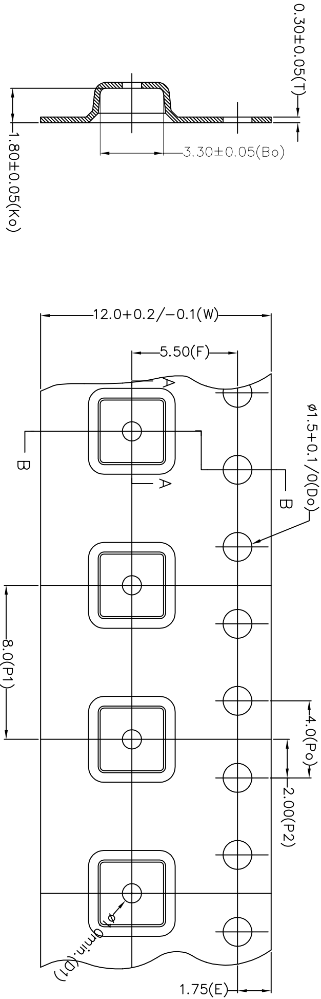
Section B-B
