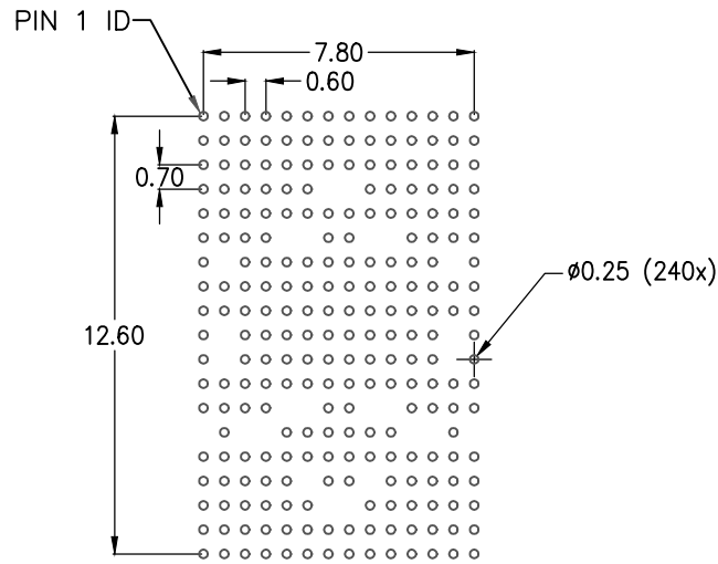
RECOMMENDED LAND PATTERN DIMENSION (TOP VIEW)
