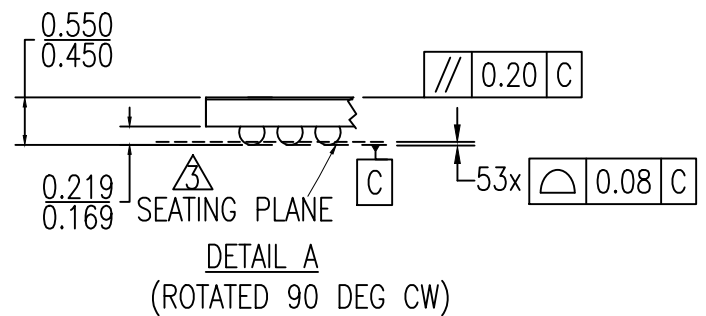
DETAIL A SIDE VIEW
