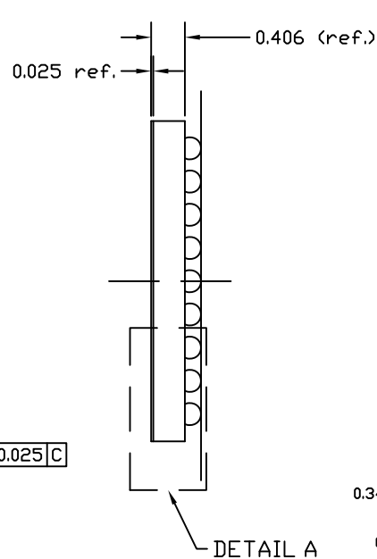
DETAIL A
