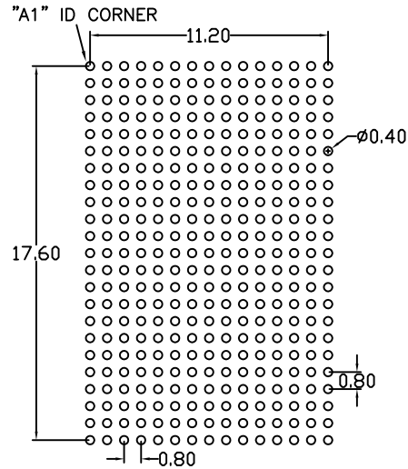
RECOMMENDED LAND PATTERN DIMENSION
