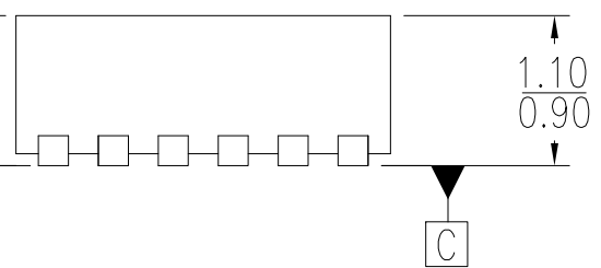
SIDE VIEW (ROTATE 90 Deg.)
